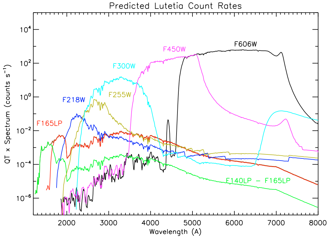
Fig. 5. After adopting our best estimate for Lutetia’s flux, we plot the predicted count rates as a function of wavelength for each of the filters employed during the HST observations. “ F140LP–F165LP ” refers to the difference between the F140LP and F165LP filters. For clarity, the F140LP curve is not explicitly labeled, but it is essentially identical to the F165LP curve longward of 1650 Å and essentially identical to the F140LP–F165LP curve shortward of that wavelength. Note the logarithmic scale.
