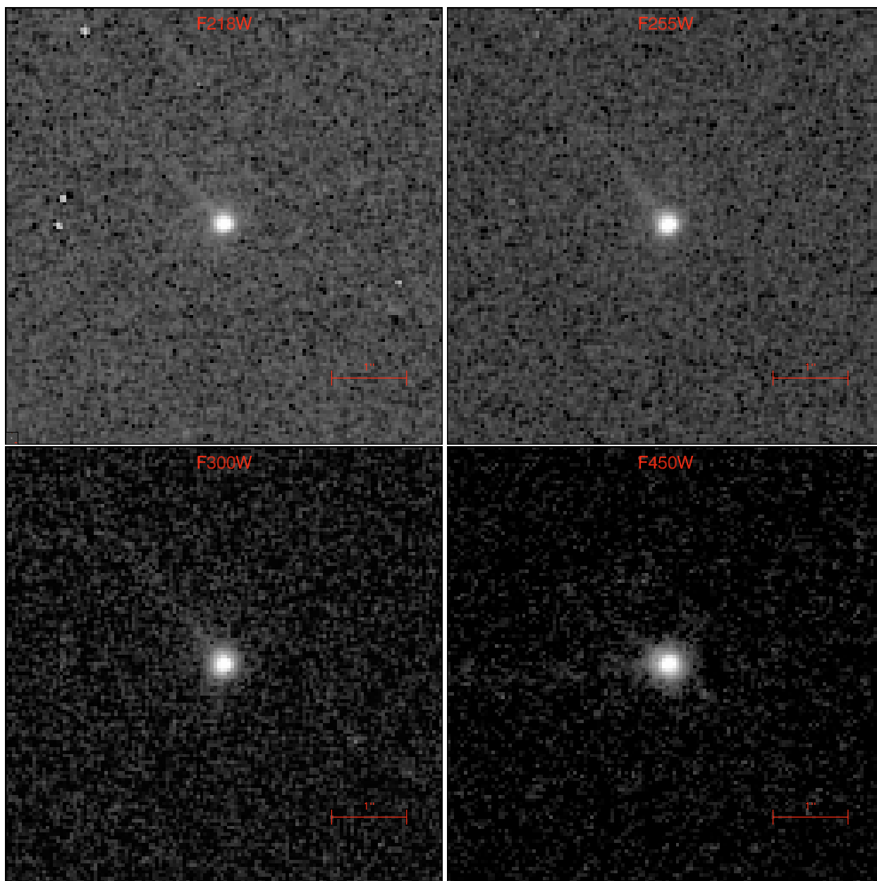
Fig. 1. HST /WFPC2 images of asteroid 21 Lutetia taken through the F218W , F255W , F300W , and F450W filters (see identifying labels on the images). Each image is a 128 \times 128 pixel subsection (each image is 5''.89 across) of the full image and is displayed using an asinh intensity stretch (similar to logarithmic) ranging from approximately zero to the maximum intensity in each image. All images have been rotated so that celestial north points up and east is to the left. The scale bar is 1'' across, which subtends 1088 km at Lutetia on December 15 (when the F450W image was taken), and 1044 km on November 30 (when all the other images were taken). Each image is a composite of at least two separate images taken with Lutetia centered at two different locations on the CCD. The “tails” apparent on two of the images are low-level artifacts caused by degraded charge transfer efficiency in the WFPC2 CCD.
