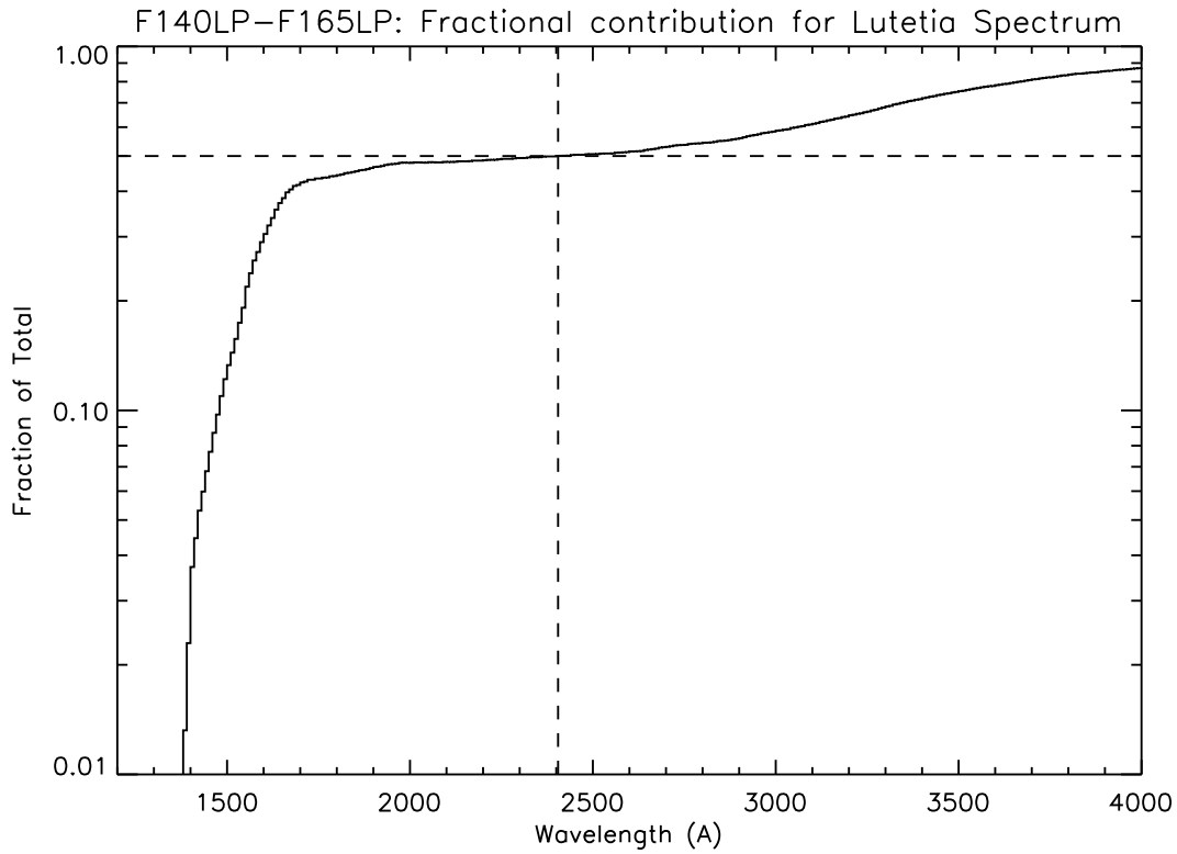
Fig. 6. The cumulative fractional contribution to the observed count rate as a function of wavelength for the difference ( F140LP–F165LP ) of the two far-UV filters employed during the HST observations. Approximately 40% of the observed signal is produced by photons having wavelengths smaller than 1675 Å, but 50% of the signal is coming from light longward of 2400 Å.
