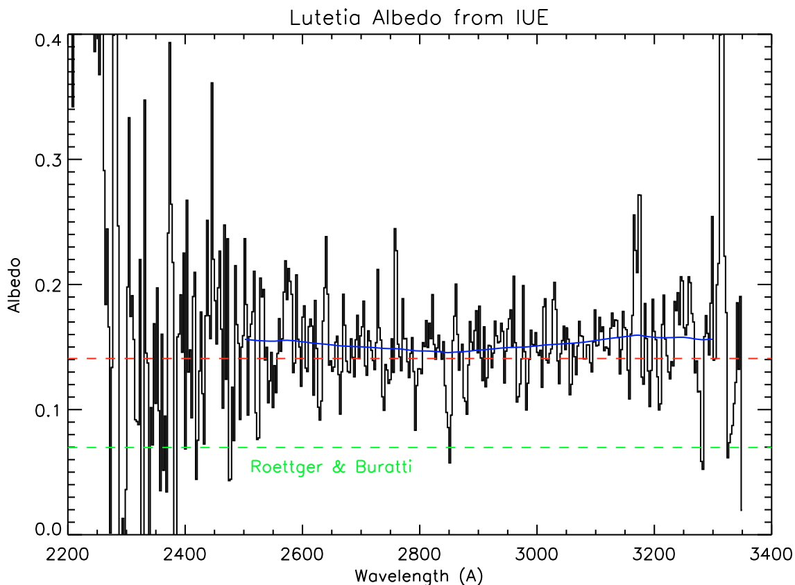
Fig. 7. Albedo spectrum of Lutetia derived from IUE observations made on 7 January 1982 at a solar phase angle of 26.1^\circ . The albedo at 2670 \text{ \AA} adopted by Roettger & Buratti (1994) is shown by the dashed green line (the lower dashed line), while our equivalent value, using a different phase correction, is depicted by the dashed red line (the upper dashed line). The blue curve is a Fourier-filtered version of the IUE spectrum, passing only the lowest 1% of spatial frequencies.
