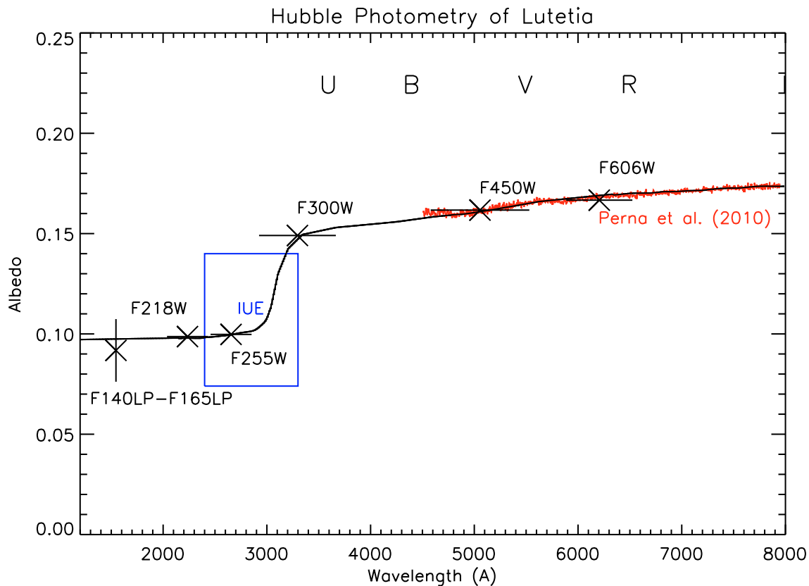
Fig. 8. Our best estimate for the albedo of Lutetia is plotted as a solid black line. The spectrum plotted in red is from a ground-based observation taken on 28 November 2008. The blue rectangle shows the wavelength coverage and the range of possible albedos derived from an IUE spectrum taken on 7 January 1982. The HST data (x) are plotted at the wavelengths where the predicted count rate is largest; the horizontal bars give the “effective bandwidth” of the filters, as specified in the STScI Instrument Handbooks. The wavelengths of the standard UBVR bands are also displayed for reference. Only the error bar for the F140LP–F165LP difference filter case is displayed because the error bars for the other filters are smaller than the plotting symbols.
